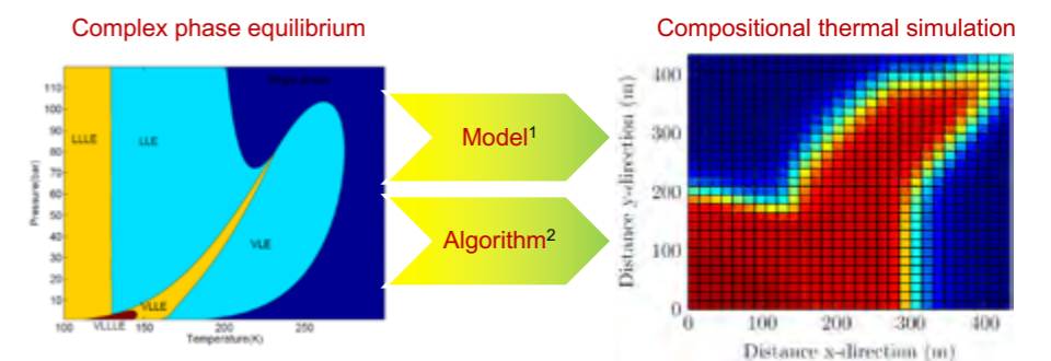
1. GE-type mixing rules and association models 2. Multiphase PH flash and new RAND formulations
