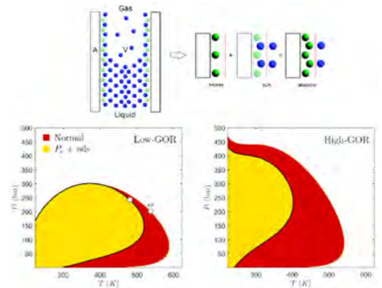
Effect of capillary pressure and adsorption on phase equilibrium of fluids with different GORs (gas oil ratios)
