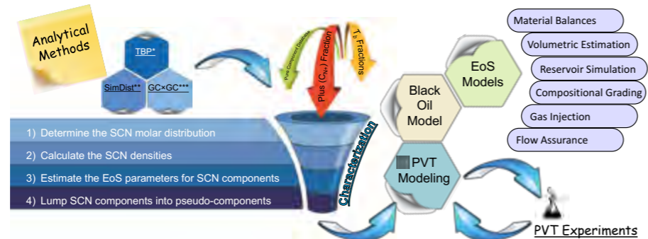
In addition to non-cubic EoS models, advanced characterization of heavy fractions is crucial to HPHT PVT modelling.
