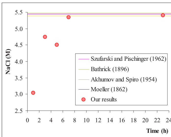
Figure 9-14. Determination of the equilibrium time for the system NaCl-H 2 O at 30°C and 1 atm when no agitation is used. M refers to molarity.
