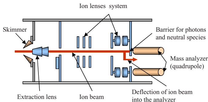
Figure 9-8. Ion lenses diagram
