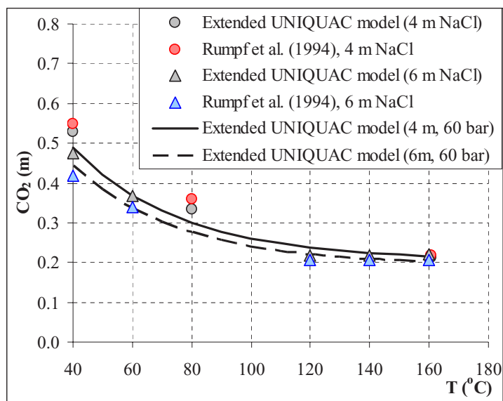
Figure 5-5. Experimental and calculated vapour-liquid phase diagram for the CO 2 -NaCl-H 2 O system at 60-70 bar. Lines represent calculations at a constant pressure of 60 bar, while grey dots and triangles represent calculations at the experimental pressure (in the range from 60 to 70 bar), which are compared to the experimental data (red and blue dots and triangles).
