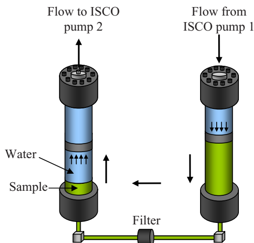
Figure 9-3. Filtration process
