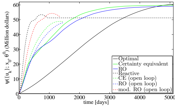
Figure 5.12: Profit evolution for the closed-loop optimization strategies. The profit evolution of the true model controlled by different strategies based on the ensemble in Fig. 5.1. Both the RO and the certainty equivalent strategies give a higher NPV than the reactive strategy. The optimal control strategy represents the best possible solution. By using the RO strategy and the certainty equivalent strategy we get profits close to the maximum possible profit.
