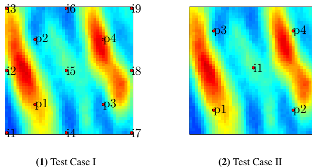
Figure 5.19: The well configuration for Test Case I and II. The permeability field in this plot is the permeability field in the upper left corner of Fig. 5.1. Producer wells are indicated by the letter p, and injector wells are indicated by the letter i. In addition to the injector and producer wells in Test Case II, Test Case I has a number of injector wells on the boundary of the field.
