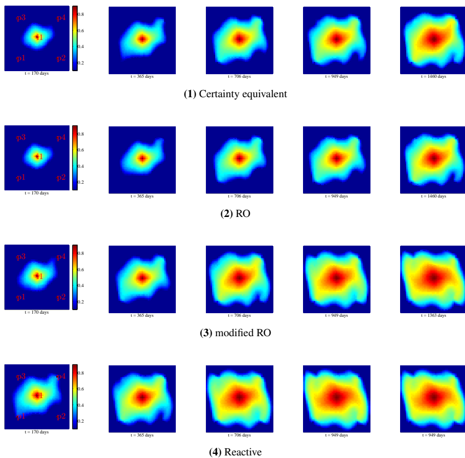
Figure 5.8: Saturation profiles of the first realization for the open-loop optimization strategies in the hundred ensemble case.
