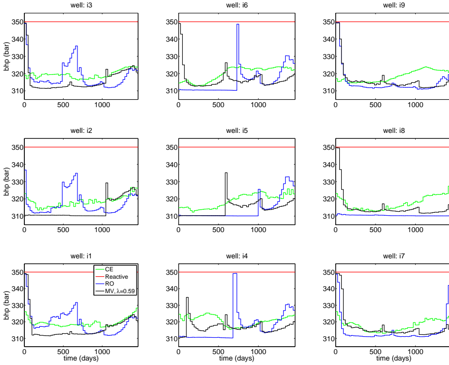
Figure 5.21: Test Case I. Trajectories of bhp for injector wells using different optimization strategies.
