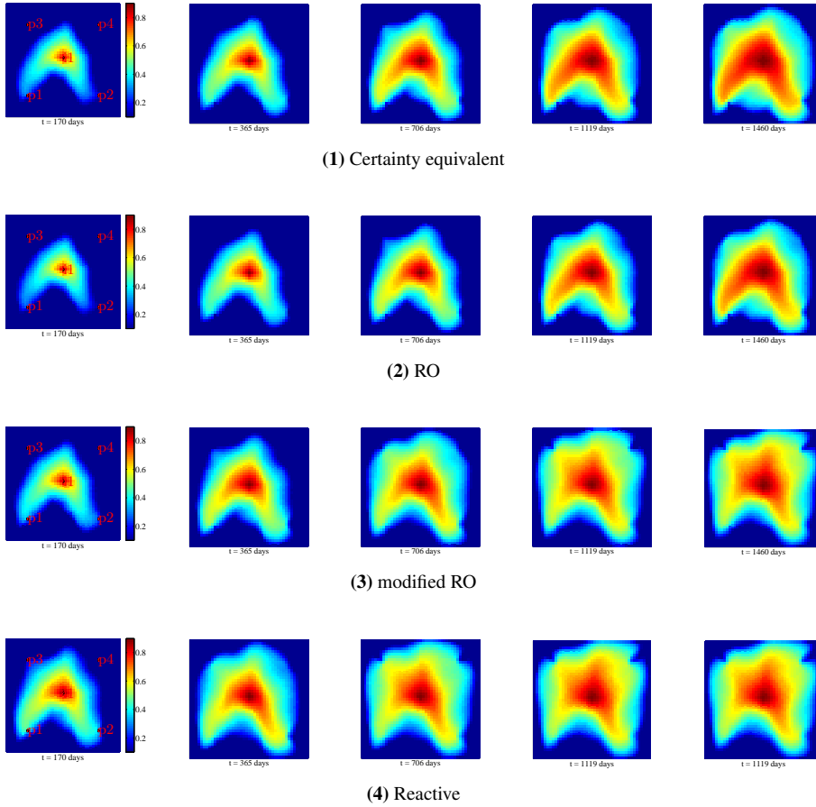
Figure 5.9: Saturation profiles of the second realization for the open-loop optimization strategies in the hundred ensemble case.
