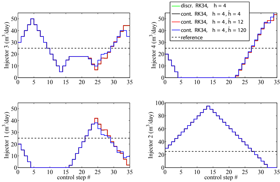
Figure 4.5: Optimal water injection rates using different adjoint methods based on ESDIRK3(4). discr.: discrete adjoint method., cont.: continuous adjoint method, h : forward step size in days, \bar{h} : adjoint step size in days.
