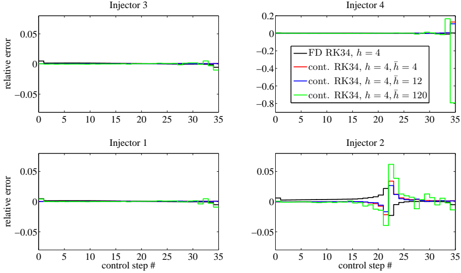
Figure 4.3: Relative error of the gradients, \frac{\partial \psi}{\partial u_k} , computed by the continuous adjoint method and the central finite difference method with respect to the gradient computed by the discrete adjoint method using a forward step size of h = 4 days. FD: Central Finite Difference, RK34: ESDIRK34, cont.: continuous adjoint method, h : forward step size, \bar{h} : adjoint step size
