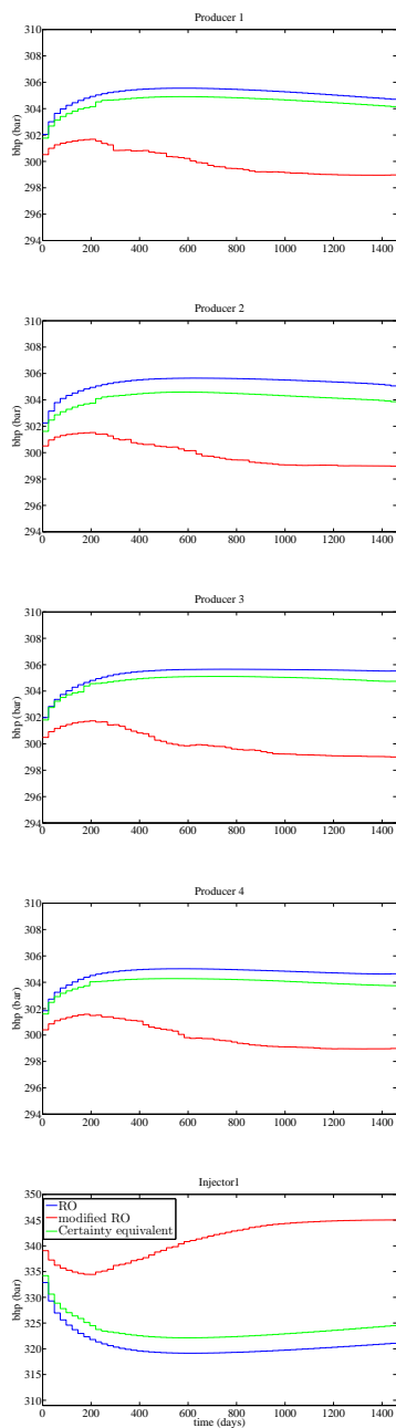
Figure 5.10: Control trajectories for open-loop optimization in the hundred ensemble case.
