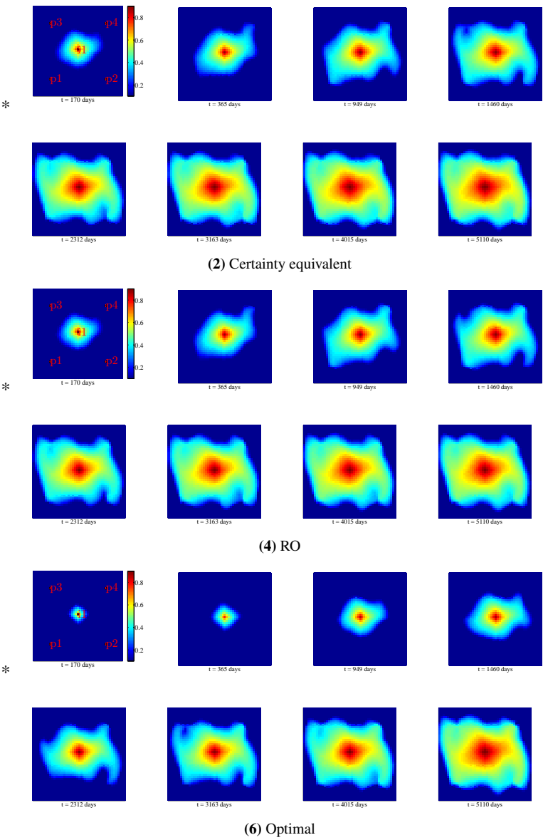
Figure 5.14: Saturation profiles of the true field for the closed-loop optimization strategies.
