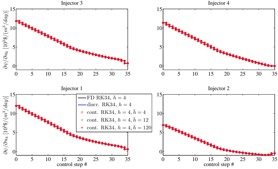
Figure 4.2: Gradient of the cost function \frac{\partial \psi}{\partial u_k} respect to the control vector. FD: Central Finite Difference, RK34: ESDIRK34, cont.: continuous adjoint method, discr.: discrete adjoint method., h : forward step size in days, \bar{h} : adjoint step size in days
