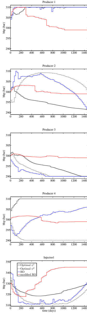
Figure 5.5: Control trajectories for open-loop optimization of the two ensemble case. The control trajectories for the considered optimization strategies are very different.
