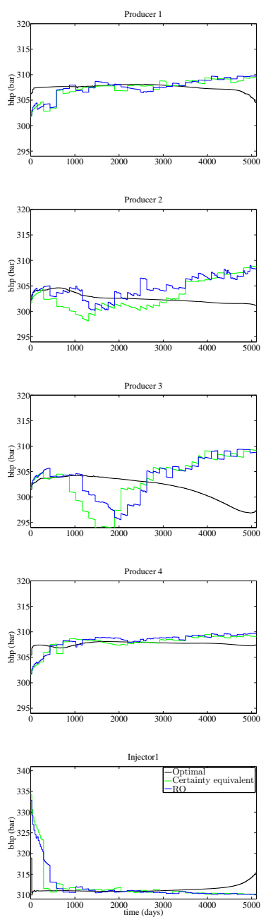
Figure 5.15: Control trajectories for the closed-loop optimization strategies.
