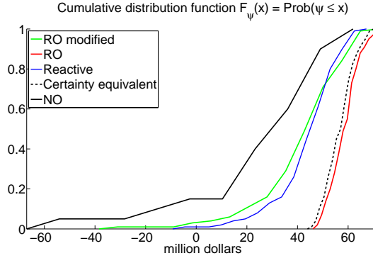
Figure 5.11: Cumulative distribution function for the open-loop optimization strategies. The cumulative distribution functions are for the ensemble with hundred members.
