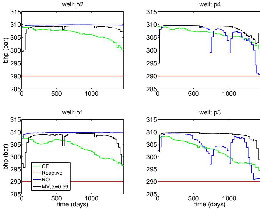
Figure 5.20: Test Case I. Trajectories of the bhp at producer wells using different optimization strategies. In the reactive strategy, the producer wells are shut in when production becomes uneconomical. The shut in time is different for each realization and is not indicated in the plot.
