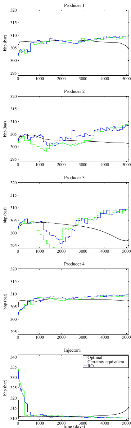
Fig. 17 Control trajectories for the closed-loop optimization strategies
