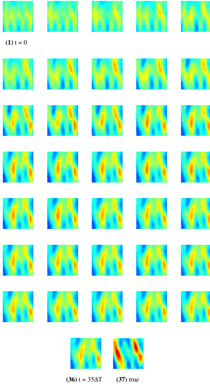
Figure 5.17: Estimates of the mean permeability field as function of time for the closed-loop certainty equivalent strategy. The initial estimate is a four channel structure. The estimates, \hat{\theta}_{k|k-1} , converge towards the true two-channel structure as more measurements are assimilated.
