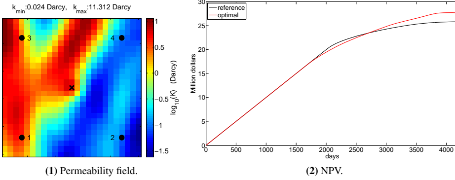
Figure 4.1: Left: Permeability field with the location of the wells. A circle indicates the location of an injector and a cross indicates the location of a producer. Right: The net present value (NPV) computed using ESDIRK3(4) and the discrete adjoint.
