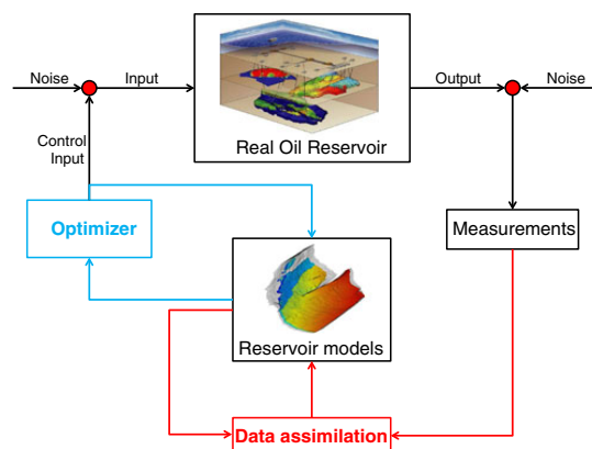
Fig. 1 Closed-loop reservoir management
