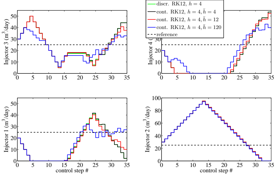
Figure 4.4: Optimal water injection rates using different adjoint methods based on ESDIRK1(2). discr.: discrete adjoint method., cont.: continuous adjoint method, h : forward step size in days, \bar{h} : adjoint step size in days.
